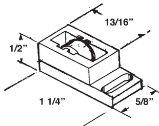
#10229 AIR CONTROL HORIZONTAL LATCH
