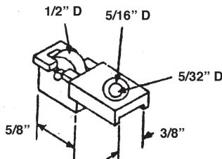
#9203 WITH BRASS WHEEL
