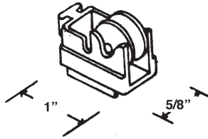
#391 HORIZONTAL WINDOW ROLLER ASSY
