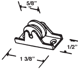
#390 HORIZONTAL WINDOW ROLLER ASSY
