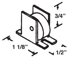
#393 HORIZONTAL WINDOW ROLLER ASSY
