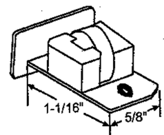
#9206 FL. EXTRUDERS WINDOW ROLLER
