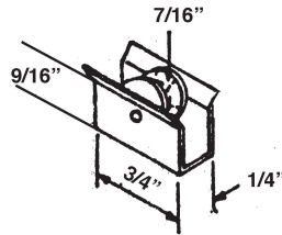
#399 HORIZONTAL WINDOW ROLLER ASSY
