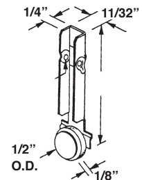
#9206 FL. EXTRUDERS WINDOW ROLLER
