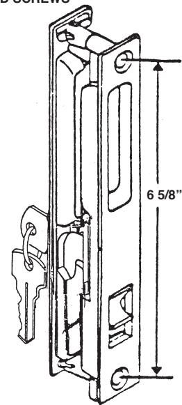
#8008 CHROME LOCK SET WITH KEY DOWNWARD LOCKING COMPLETE WITH KEEPER AND SCREWS
