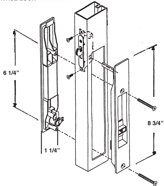
#10020 PLASTIC HOUSING #10023 WITH KEY LOCK ADAMS RITE #4431 COMPLETE SET WITH MORTISE LOCK
