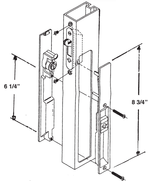
#10021 METAL HOUSING #10024 WITH KEY LOCK ADAMS RITE #4190 COMPLETE SET WITH MORTISE LOCK
