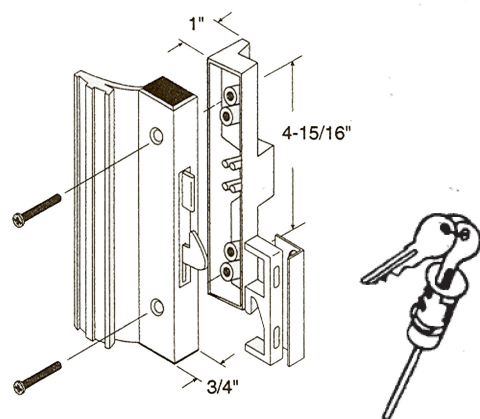
#446 UNIVERSAL SURFACE MOUNT LOCK SET WITH HOOK LATCH - WITH KEY
