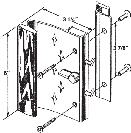
#10638 LOOK-HILITE PATIO DOOR LOCK WITH DOUBLE HOOKS
