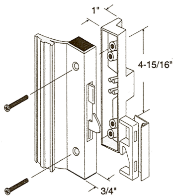
#447 UNIVERSAL SURFACE MOUNT LOCK SET WITH HOOK LATCH
