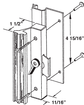
#10642 NEW LOOK PATIO DOOR LOCK SURFACE MOUNT WITH CLAMP LATCH
