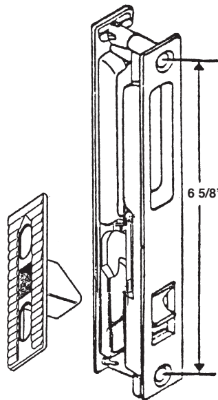
#8007B BRONZE LOCK SET DOWNWARD LOCKING COMPLETE WITH KEEPER AND SCREWS
