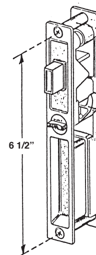
#1200 CROSSLY LOCK
