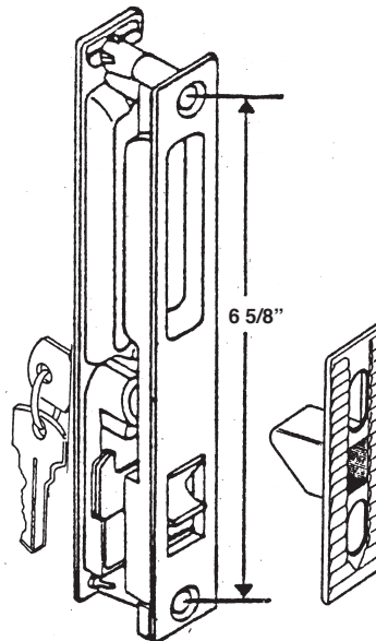
#445W WHITE LOCK SET WITH KEY COMPLETE WITH KEEPER AND SCREWS
