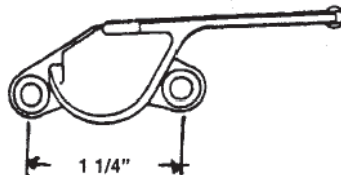
#364 KINCO SHW SASH LOCK
