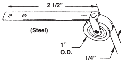
#630 SCREEN DOOR ROLLER ASSY STEEL WHEEL
