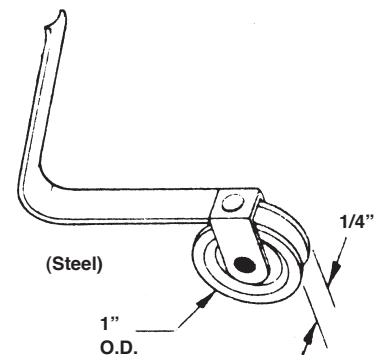
#635 SCREEN DOOR ROLLER ASSY
