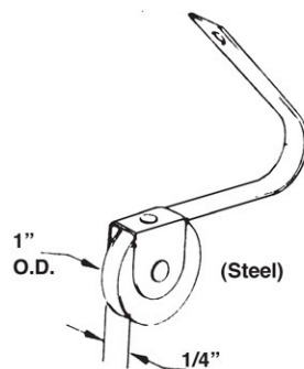
#562 SLIDING SCREEN DOOR ROLLER ASSY
