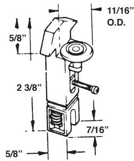
#573 SLIDING SCREEN DOOR ROLLER ASSY
