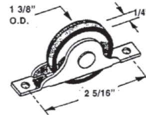
#1000 GARAGE DOOR SCREEN ROLLER
