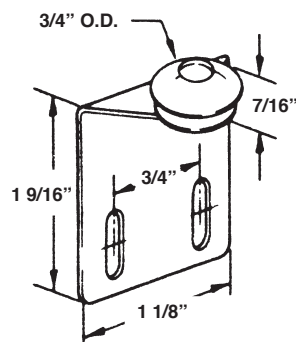
#630 SCREEN DOOR ROLLER ASSY STEEL WHEEL
