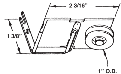
#635 SCREEN DOOR ROLLER ASSY
