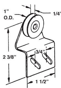
#574 SLIDING SCREEN DOOR ROLLER ASSY
