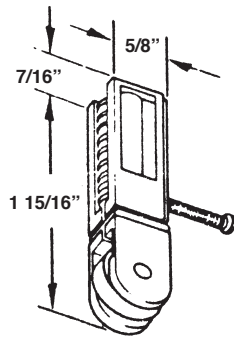
#572 SLIDING SCREEN DOOR ROLLER ASSY
