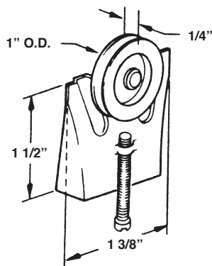
#578 SLIDING SCREEN DOOR ROLLER ASSY
