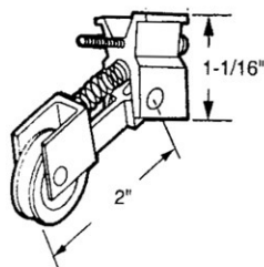
#77 MILLER SCREEN DOOR WHEEL ASSY
