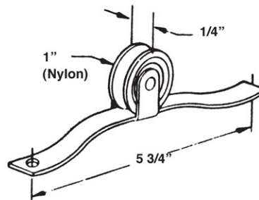
#569 SLIDING SCREEN DOOR ROLLER ASSY
