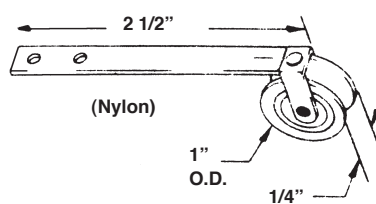
#631 SCREEN DOOR ROLLER ASSY NYLON WHEEL
