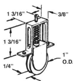
#666 SCREEN DOOR ROLLER ASSY NYLON WHEEL
