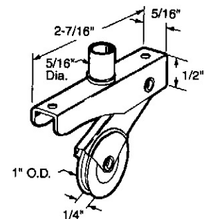
#1081 ROLLER ASSY. WITH SCREW GUIDE STEEL WHEEL #1082 NYLON WHEEL
