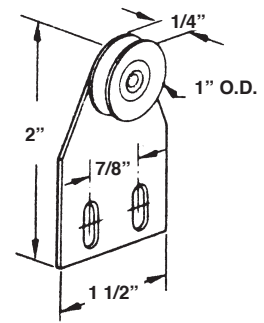
#576 SLIDING SCREEN DOOR ROLLER ASSY
