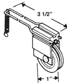
#79 DARYL SCREEN DOOR WHEEL ASSY
