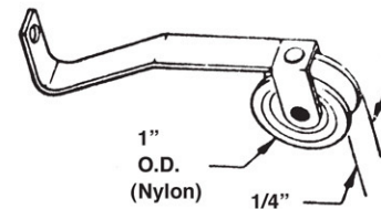
#561 SLIDING SCREEN DOOR ROLLER ASSY - NYLON WHEEL
