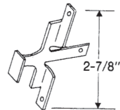
#10407 AIRPLANE LATCH
