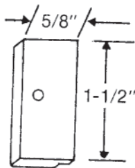
#10408 PLASTIC LATCH
