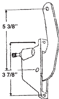
#787 LUDMAN OPERATOR L.H.
