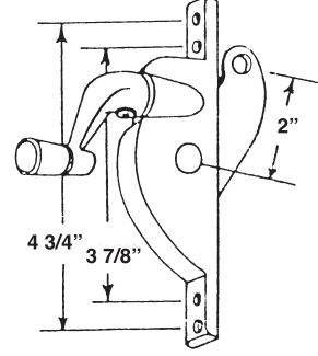
#791 D-8 L.H. JTW OPERATOR
