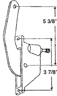
#1104 ABC LINK
