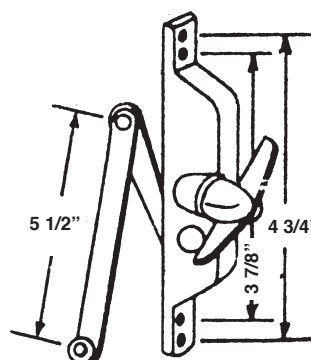
#260 5 1/2" JALOUSIE OPERATOR
