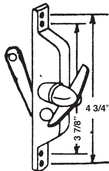
#261 UNIVERSAL JALOUSIE OPERATOR
