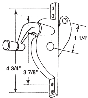
#787 LUDMAN OPERATOR L.H.
