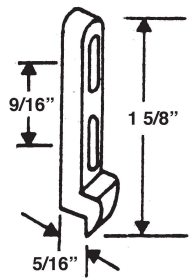
#677 SCREEN DOOR KEEPER
