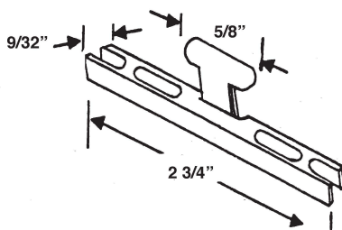
#339 YALE SCREEN DOOR KEEPER
