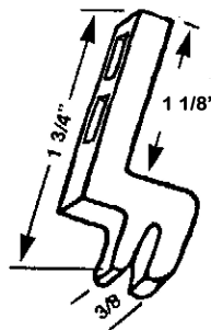
#708 PLASTIC SCREEN DOOR KEEPER
