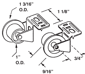
#413 WHEEL GUIDE ASSY. (1 PR.)
