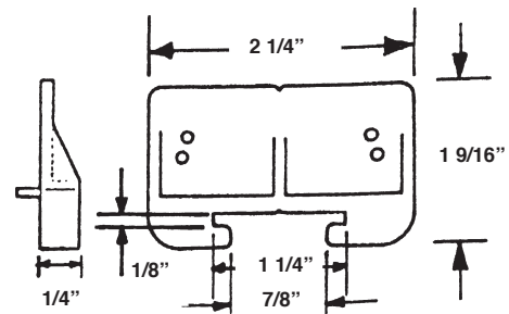
#425 NYLON DRAWER SLIDE
