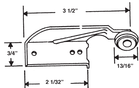
#422 DRAWER BRACKET & WHEEL GUIDE
