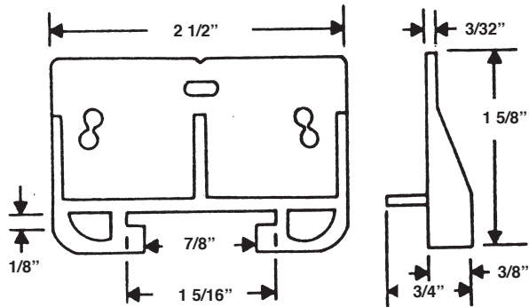
#407 DRAWER NYLON SLIDE
