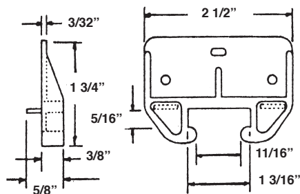
#420 DRAWER TRACK SLIDE GUIDE
