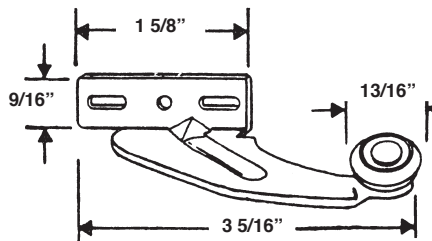
#421 DRAWER BRACKET & WHEEL
