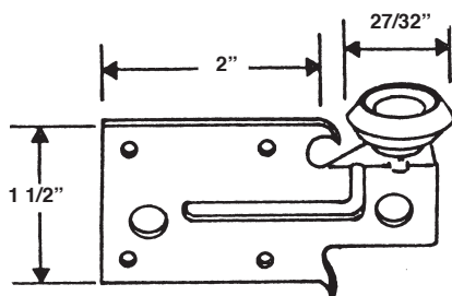
#411 DRAWER BRACKET & WHEEL
