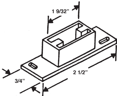
#417 TRACK REAR BRACKET
