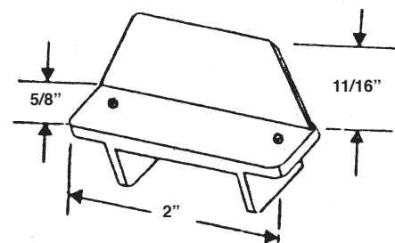
#422 DRAWER BRACKET & WHEEL GUIDE
