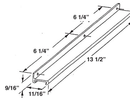
#10601 WOOD CASEMENT WINDOW REPLACEMENT TRACK
