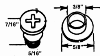
#192 SHOULDER BOLT & BUSHING
