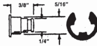
#201 1/4" RIVET & "E" RING
