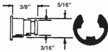
#200 3/16" RIVET & "E" RING
