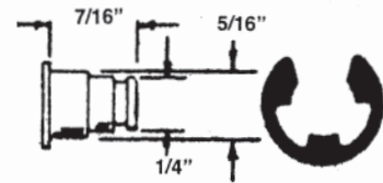
#202 1/4" RIVET & "E" RING
