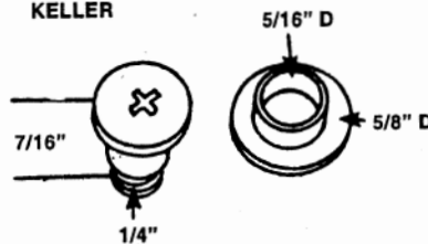
#191 SHOULDER BOLT & BUSHING KELLER
