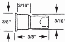
#204 RIVET FOR HARCAR VENT LOCK
