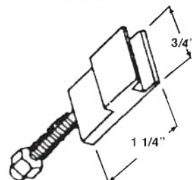
#10385 OLD PAN AM SCREEN DOOR GUIDE
