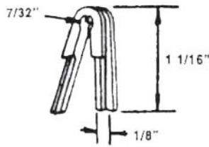
#483 DARYL TOP RAIL GUIDE
