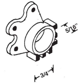
#912 TORQUE BEARING
